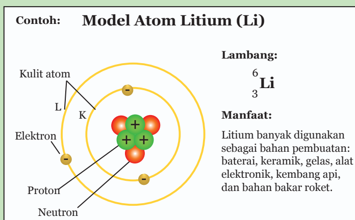
Gambar 8.2 Model Atom Litium (Li)
